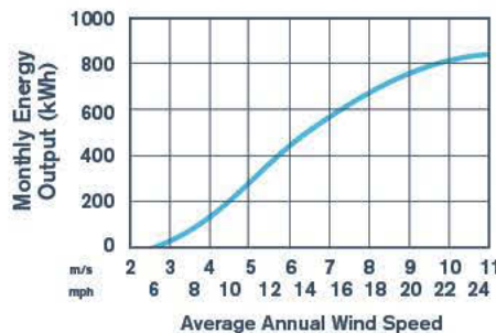
MONTHLY ENERGY
